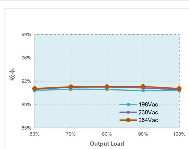
Fig.6 Efficiency-Load curve
